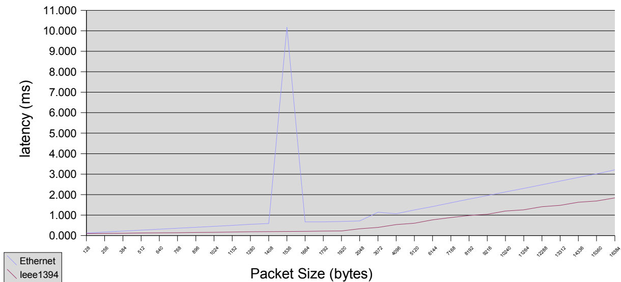
Latency: ieee1394 vs. Ethernet(100m)
